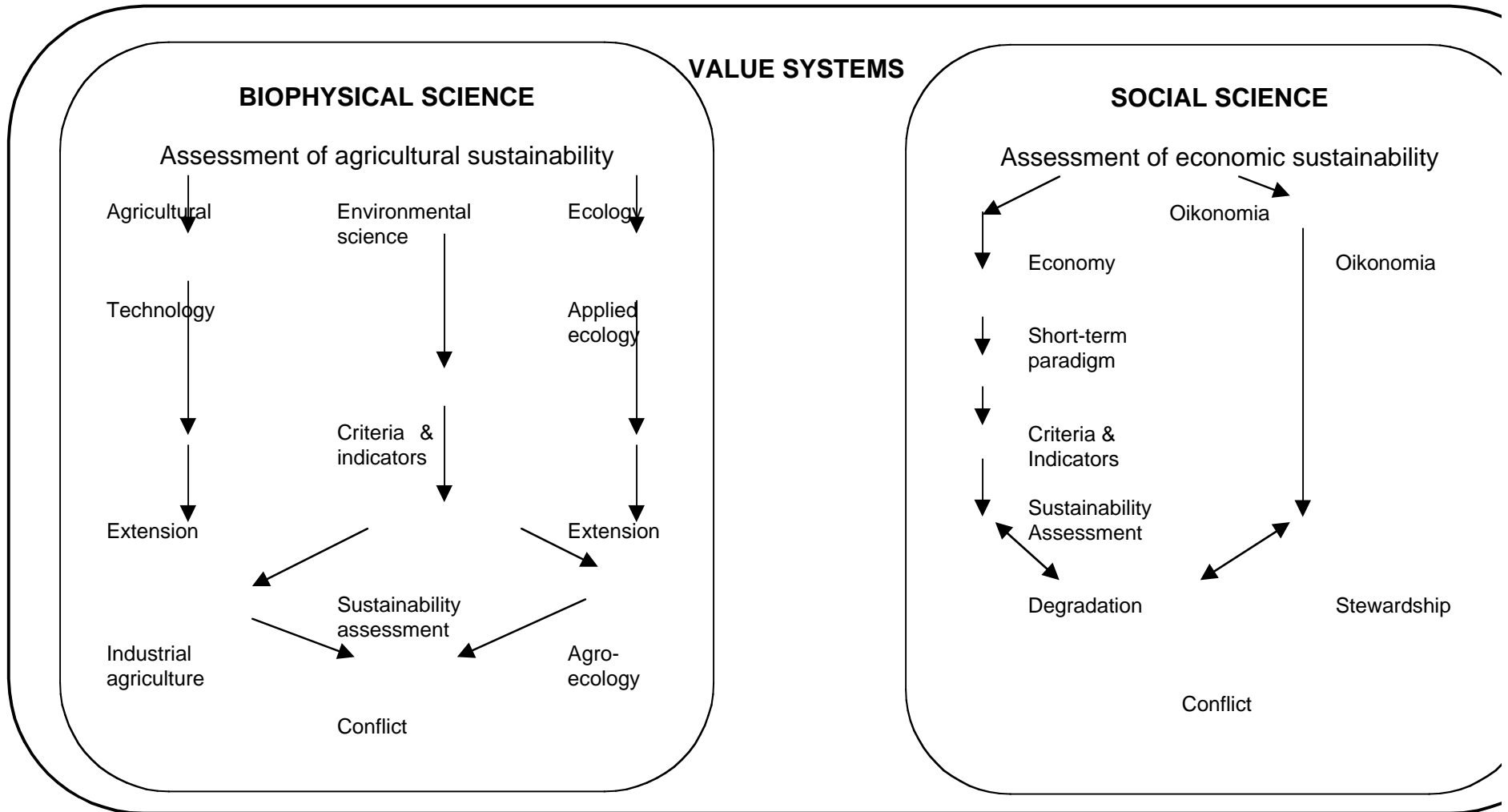
Figure 1 Conflicts between elements of sustainability assessment in agriculture
